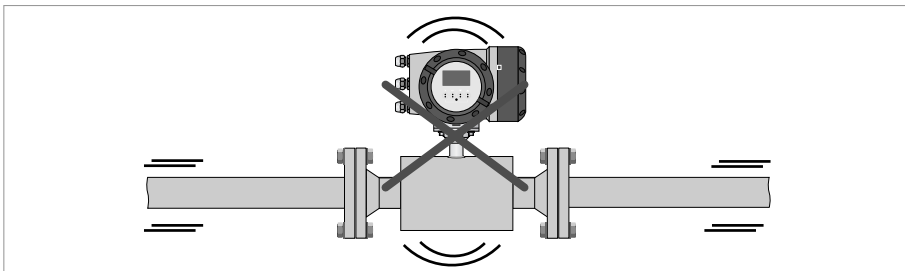
Figure 2-5: Avoid vibrations
