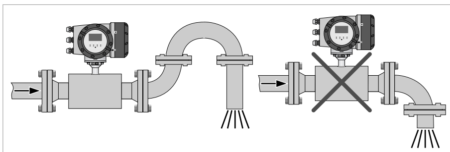
Figure 2-11: Open discharge
