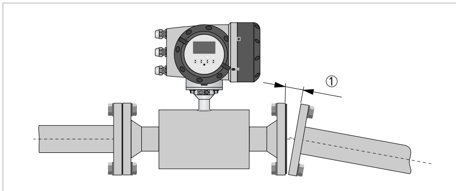
Figure 2-16: Flange deviation
